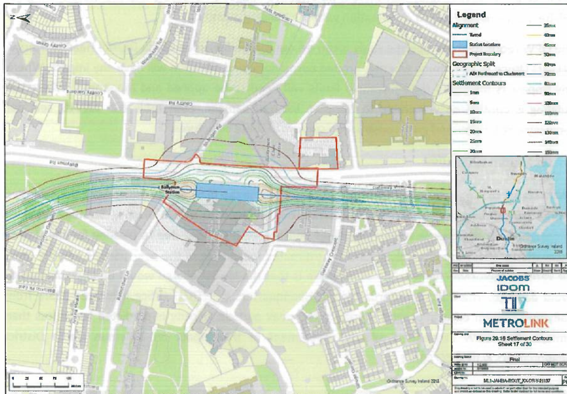
Figure 8. Settlement Contours (Extract from ML1-JAI-EIA-ROUT_XX-DR-Y-21137)
